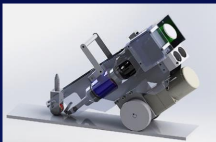
[AUTO PFA WELDING M/C(BAND)]
