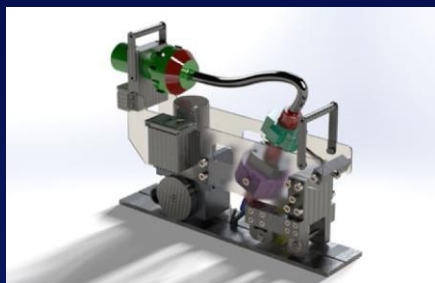
[AUTO PFA WELDING M/C(ROD)]
